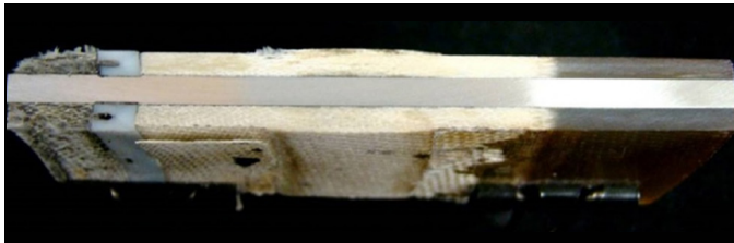
Steam attack on GRE isolation gasket
